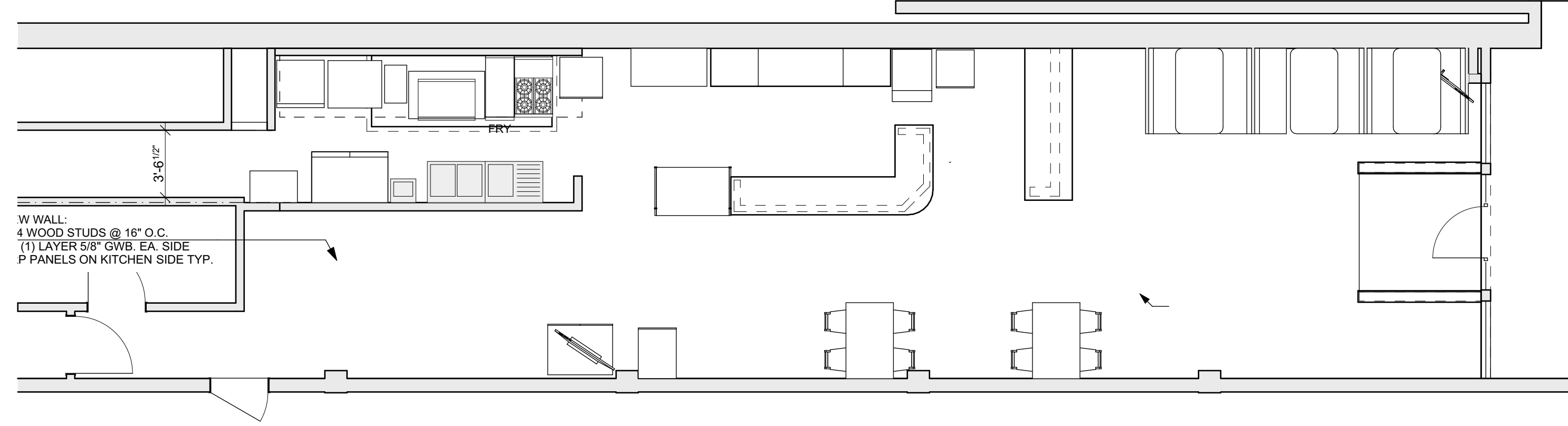
1 EXISTING FLOOR PLAN SCALE: 3/16" = 1'-0"
