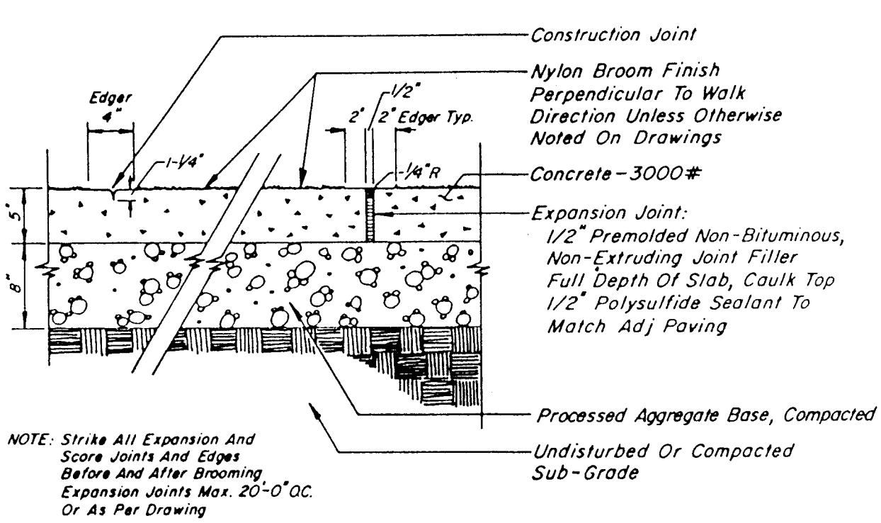
CONCRETE PAVING SCALE 1" = 1'-0"
