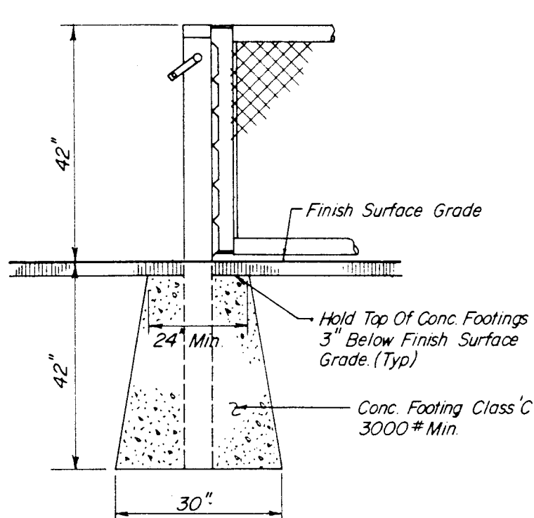
NET POST DETAIL
