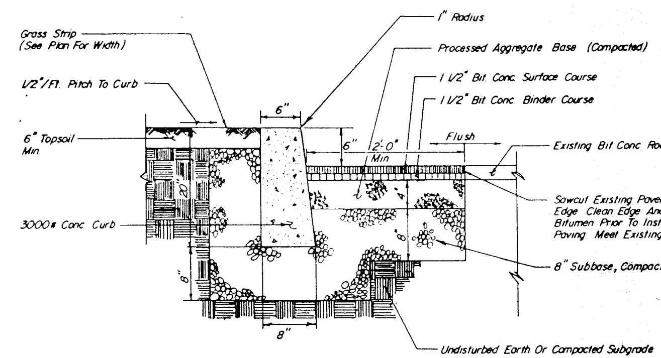
CONCRETE CURB
