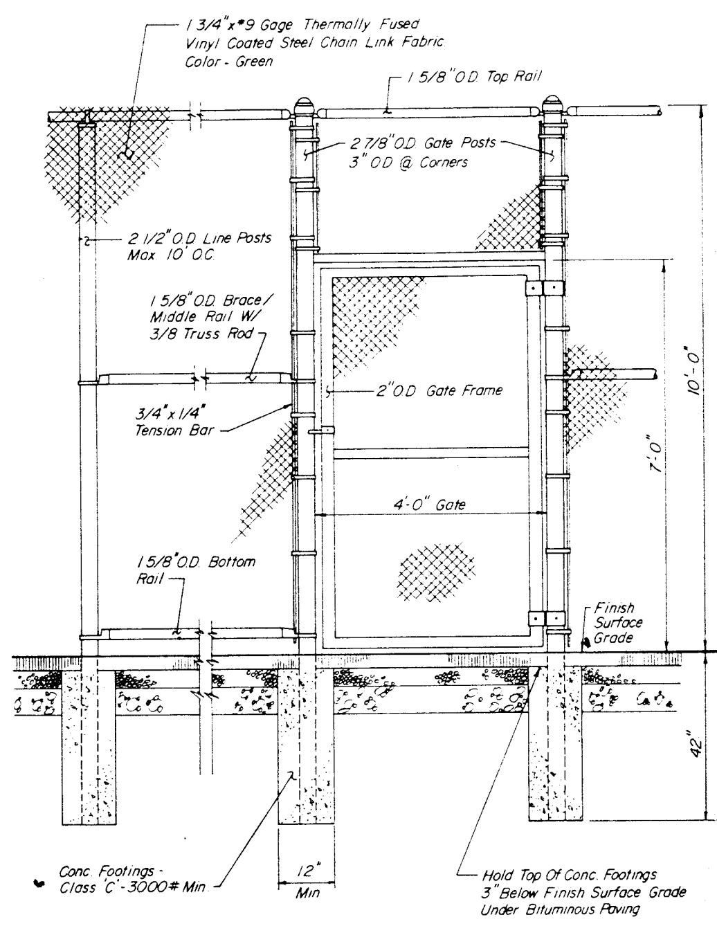
FENCE DETAIL
