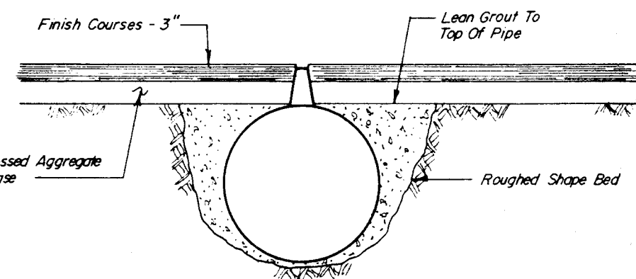
SLOTTED CMP DRAIN PIPE DETAIL
