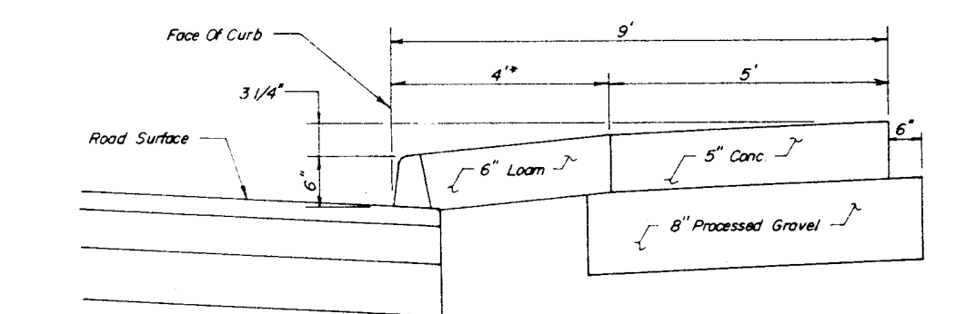
SECTION TYPICAL SIDEWALK NTS
