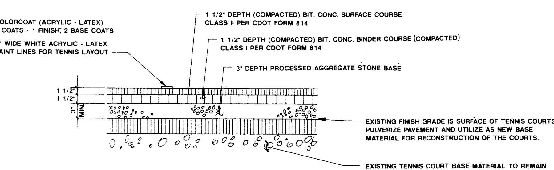
TYPICAL SECTION THROUGH COURTS SCALE: 1" = 1'
